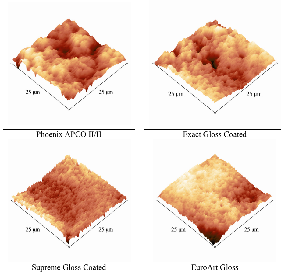
Figure 13. The AFM pictures of the surface of the tested papers.
