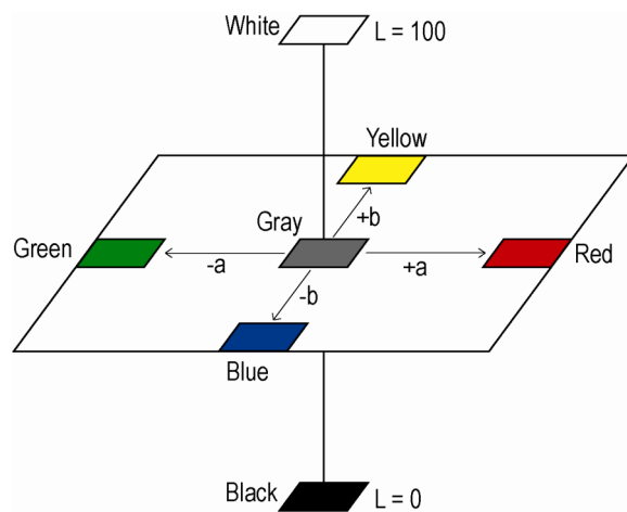
Figure 3. The CIE L^*a^*b^* colour scale (Based on Field, 1999).
