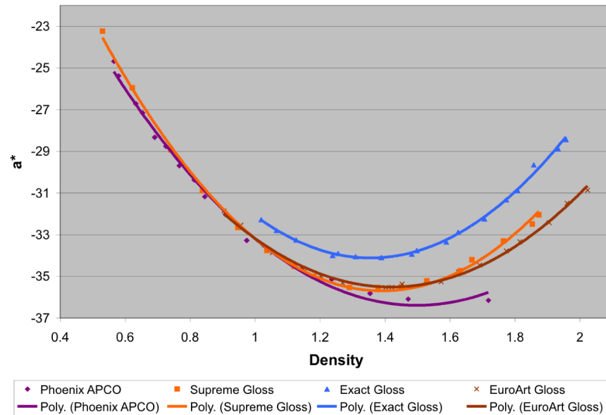
Figure 5. Density versus a^* for cyan printed on coated stocks.
