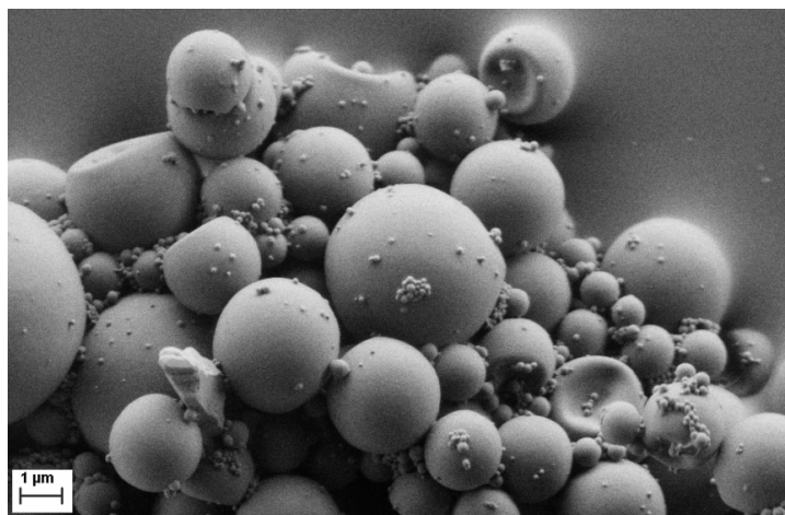
Figure 1. SEM micrograph of a TC pigment powder. Most particles are circular-shaped capsules with diameter of several µm. The irregular particles are non-encapsulated composite.
