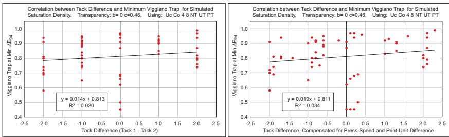
Figure 7a and 7b. Correlation between tack and minimum Viggiano Trap.
