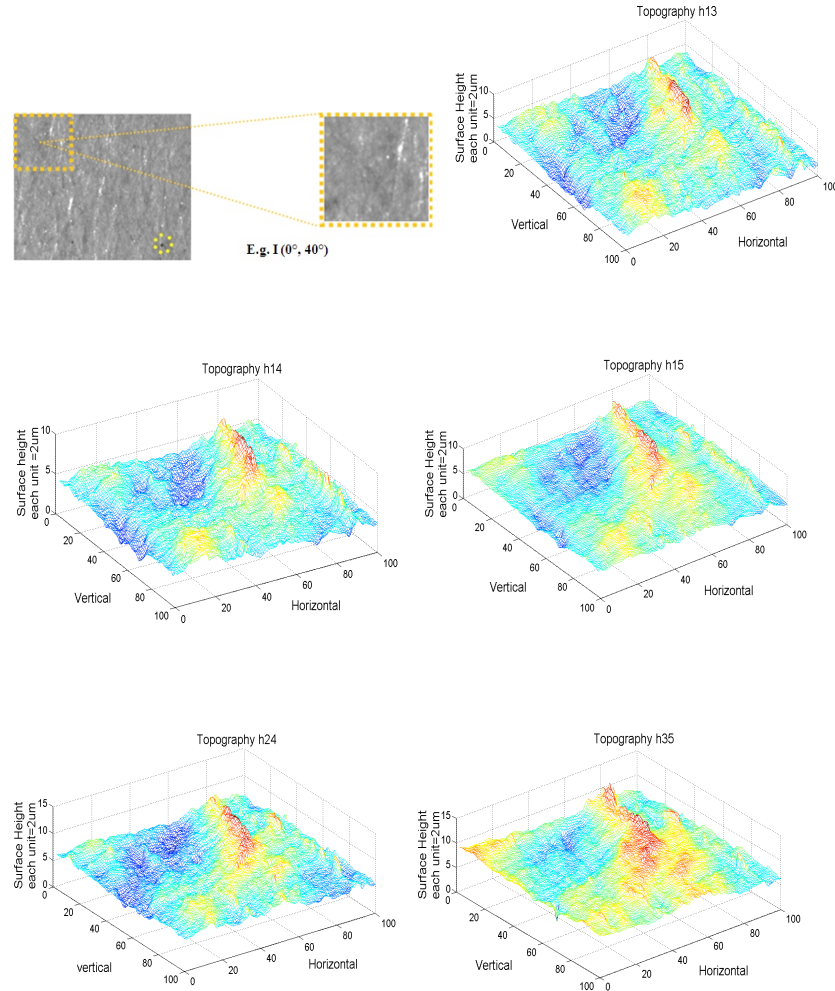
Figure 4. 5 different groups of images were chosen to do the calculation, the calculated surface topography of the same paper sample were shown, the displayed size is 200 \mu\text{m} \times 200 \mu\text{m} .
