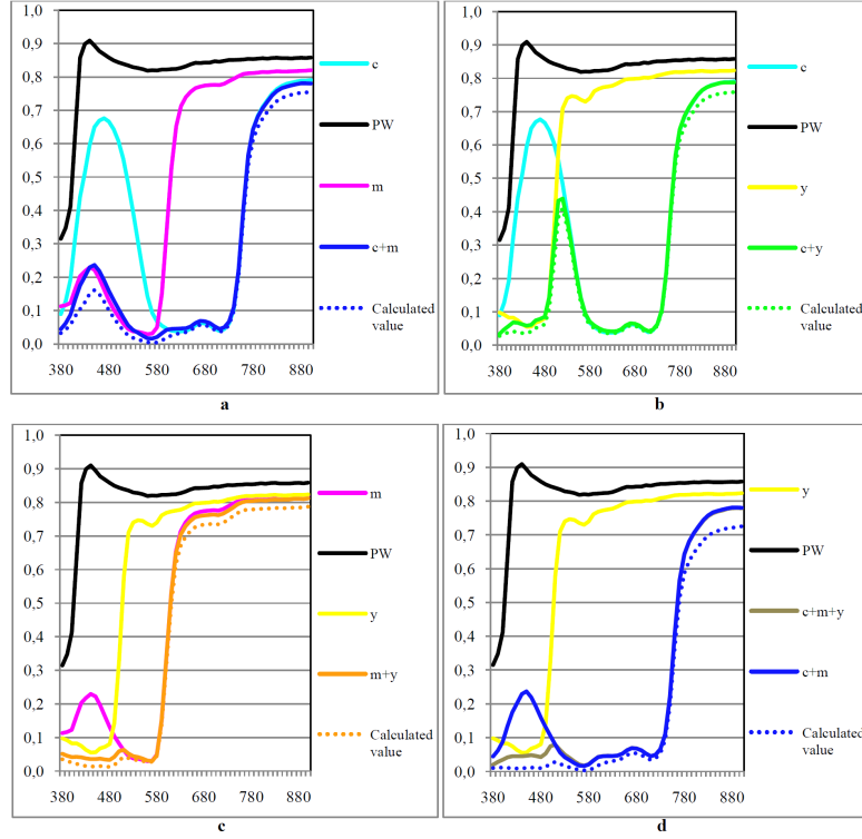
Figure 3. The spectral reflectance curves of the overlapped and calculated inks. c denotes cyan, m magenta, y yellow, c+m measured the overlapping of magenta on cyan, c+y measured the overlapping of yellow on cyan, m+y measured the overlapping of yellow on magenta, c+m+y measured the overlapping of yellow on blue. The dashed lines are the corresponding spectral curves of calculated overlapping. PW is the spectral reflectance of the paper.
