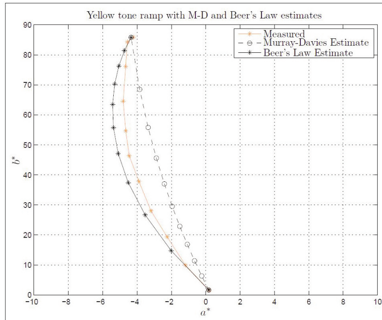
Figure 12: Yellow tone ramp, web offset, conventional and stochastic screens and Murray- Davies and Beer's Law estimates, coated matte paper.
