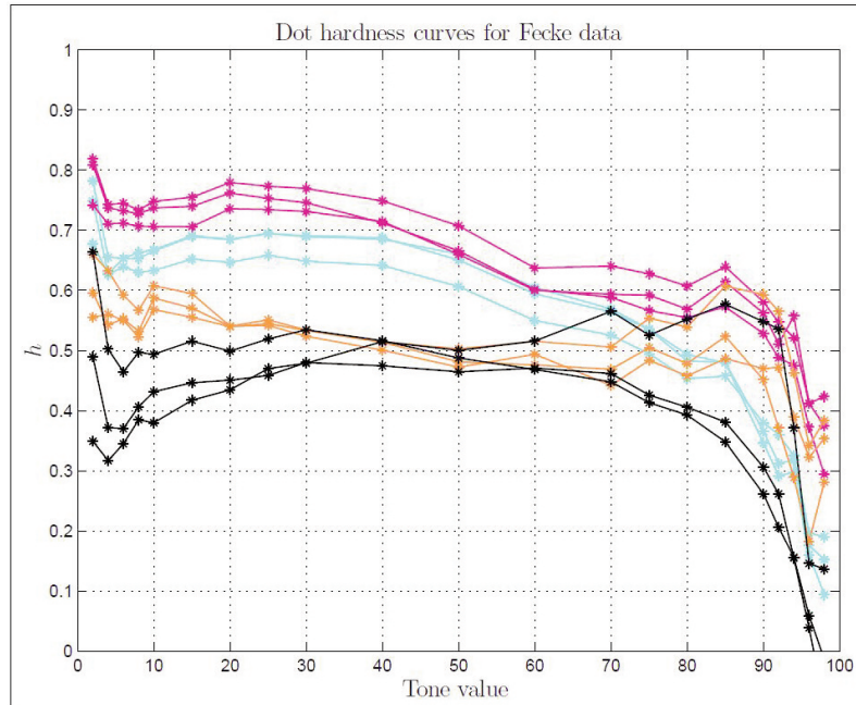
Figure 34: Dot hardness vs. tone value, Fecke data.
