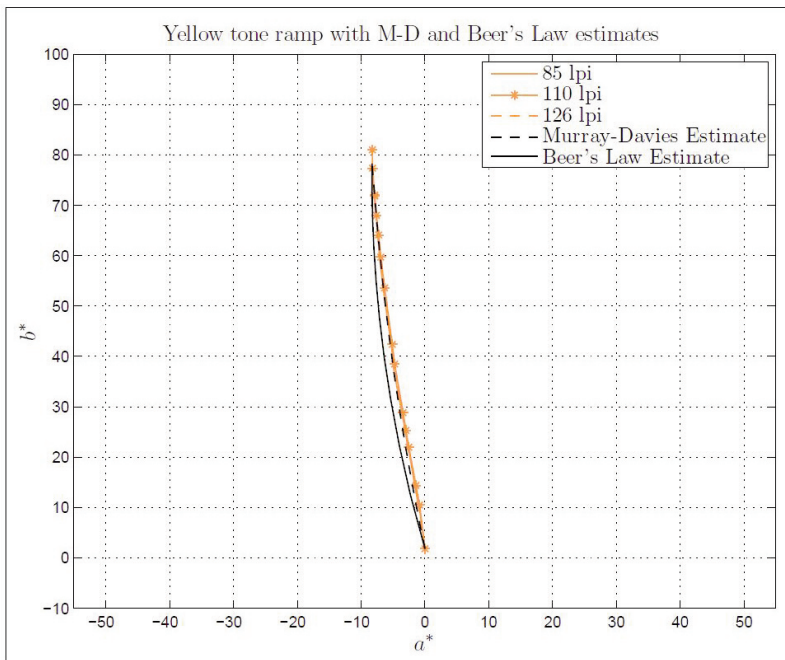
Figure 18: Yellow tone ramp, flexo data and Murray-Davies and Beer's Law estimates.
