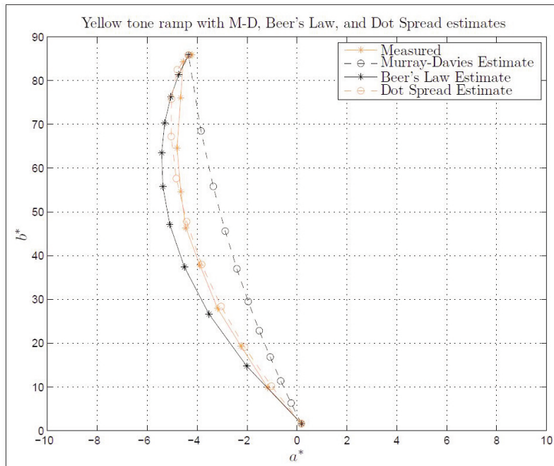
Figure 27: Cyan, magenta, yellow tone ramps, \Delta E^*_{ab} values of the dot spread estimate, coated matte data.
