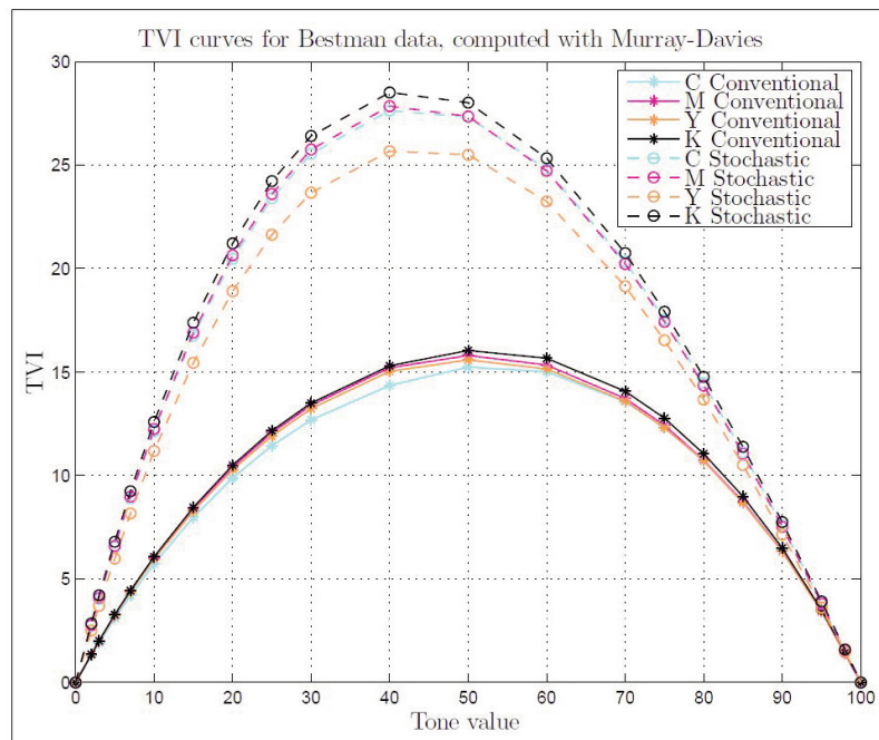
Figure 36: TVI curves for Bestman data, conventional and stochastic line screens.
