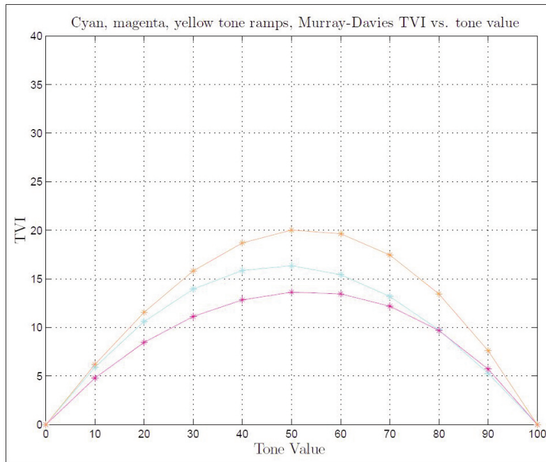
Figure 21: Cyan, magenta, yellow tone ramps, best-fit Murray-Davies TVI vs. tone value, coated matte data.
