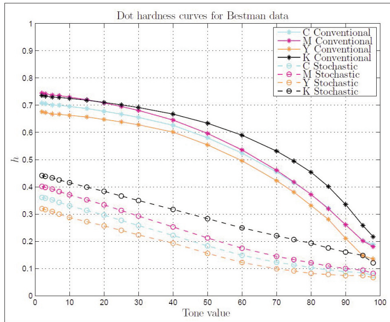
Figure 38: Dot hardness vs. tone value, Bestman data.
