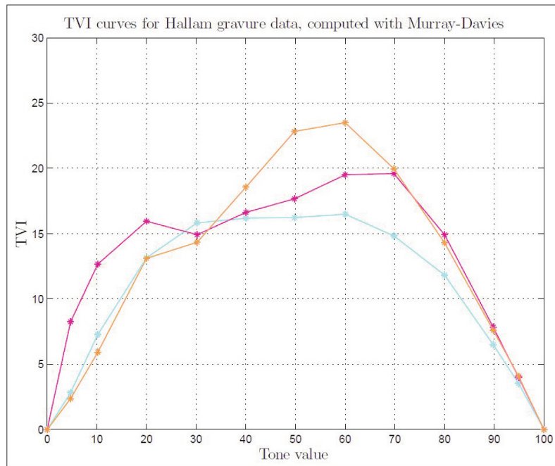
Figure 40: TVI curves for Hallam gravure data.
