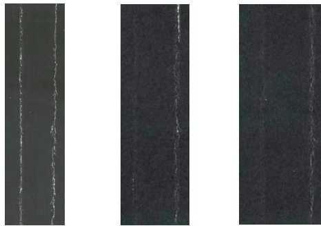
Figure 1: Printed and folded paperboards with aqueous coating applied. Folding lines were scanned with an Epson scanner. The left one was printed with Ricoh C900S. The paperboard was not corona treated. The middle one was printed with HP Indigo 3050 on the untreated paperboard. The right one was printed with HP Indigo 3050 on the corona treated paperboard.
