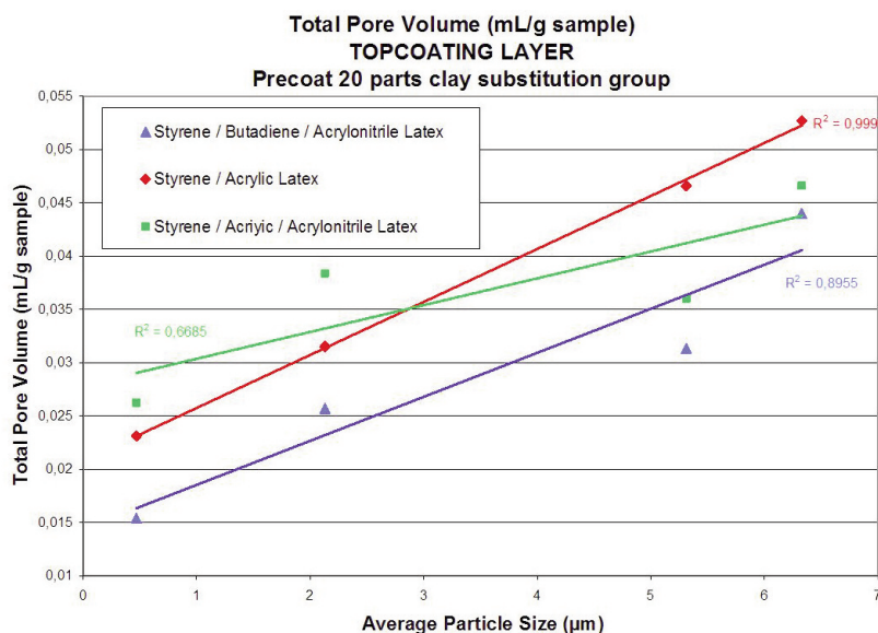
Figure 9 - Total Pore Volume (TPV) Topcoated layer for Group 1 as a function of the particle size of the precoat layer – Comparison of the 3 latexes.
