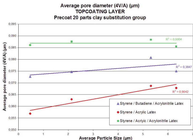
Figure 10 - Average Pore Diameter (APD) Topcoated layer for Group 1 as a function of the particle size of the precoat layer – Comparison of the 3 latexes.
