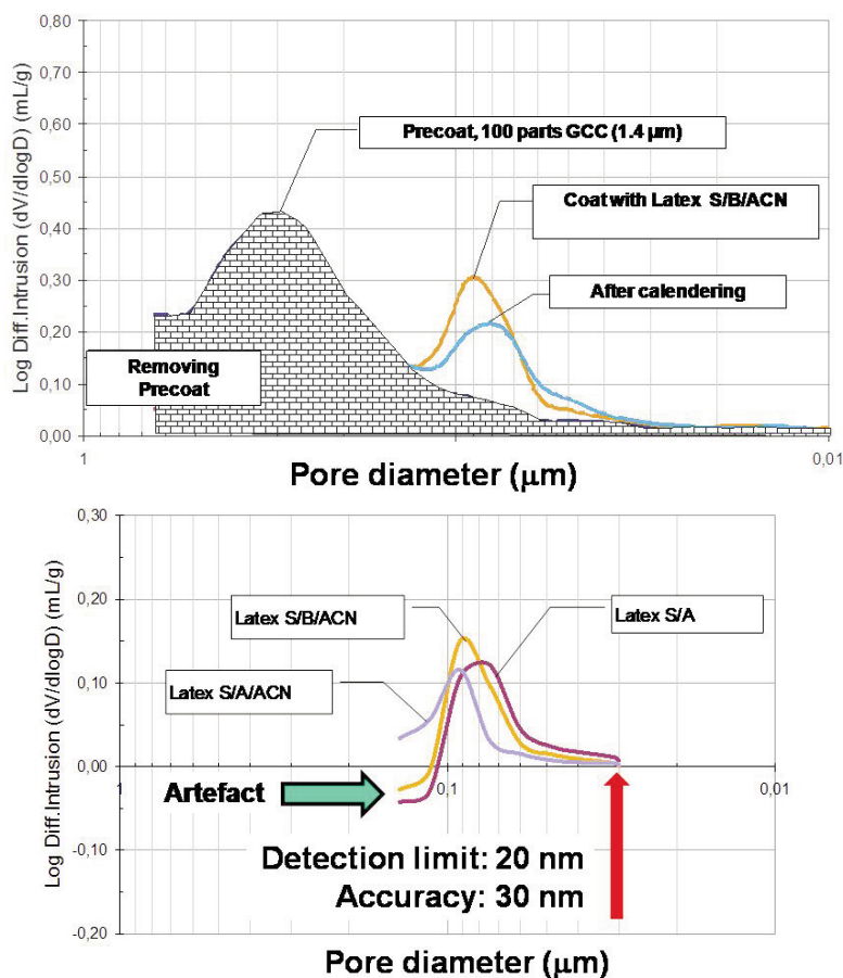
Figure 5 - Schematic illustration of the procedure used for removing the pore data related to the precoat. After precoat data removal the negative values obtained for the topcoat above 0.1 \mu\text{m} are mathematical artefacts.
