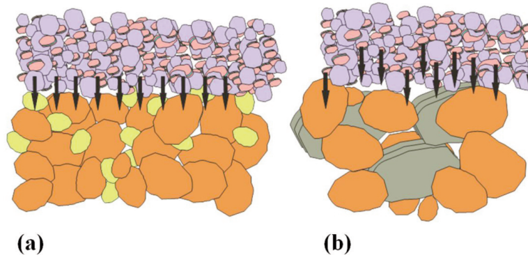
Figure 11 – (a) Capillary theory related to smaller pores in the precoat. Topcoat: GCC is in purple-blue, clay in light red. Precoat: GCC is in orange and N°1 fine clay is in yellow. (b) Preferential movement theory related to bigger pores in the precoat. Topcoat: GCC is in purple-blue, clay in light red. Precoat: GCC is in orange and high aspect ratio clay is in grey.
