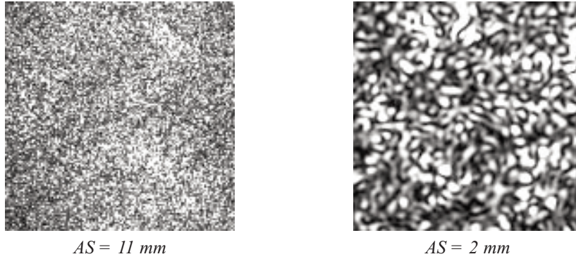
Figure 4: Speckle patterns captured at different aperture sizes (AS). The image size was 128x128 pixels.
