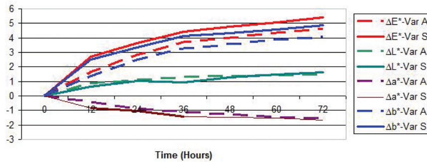
Figure 7: Experimental Phase II - Change in CIELAB values for FWA paperboard samples after UV varnishing (both varnish A and S).
