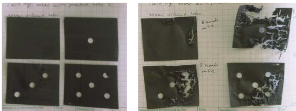
Figure 6. Early stages of printed susceptor pattern, before (left) and after (right) microwave cycle.
