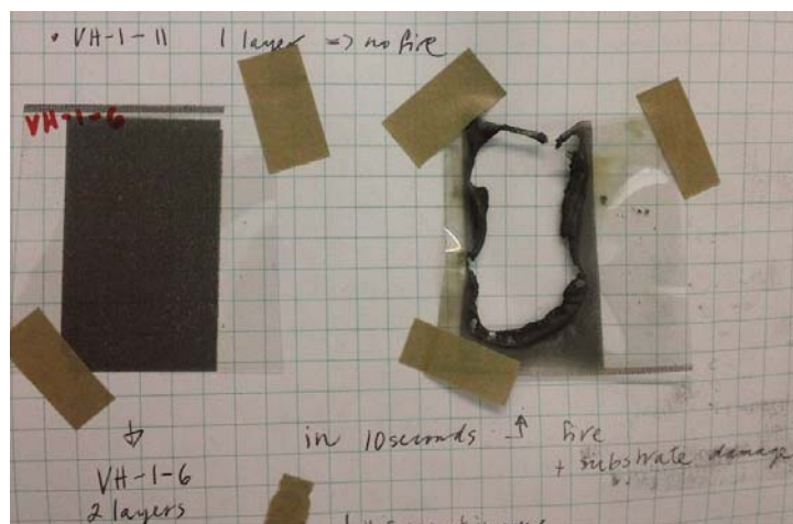
Figure 8. Susceptor constructed out of 2 layers on the left. Same susceptor after 10 seconds in microwave oven.
