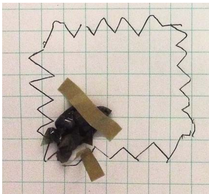
Figure 7. Susceptor ink resulted in shrinking of PET. Outline represents original design and size of the susceptor.
