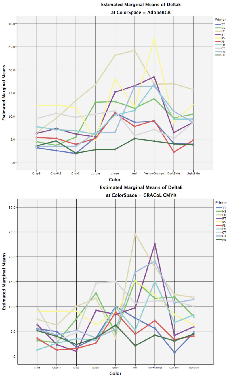
Figure 21,22: Graphs showing the mean \Delta E for each company for each of the nine measured color patches. The top graph shows the AdobeRGB file readings and the bottom graph shows the GRACoL CMYK readings
