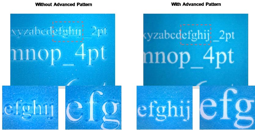
Figure 7 – Images showing at 200X magnification the impact of Advanced Edge Definition (AED) with fine text reverses for solvent based ink on film
