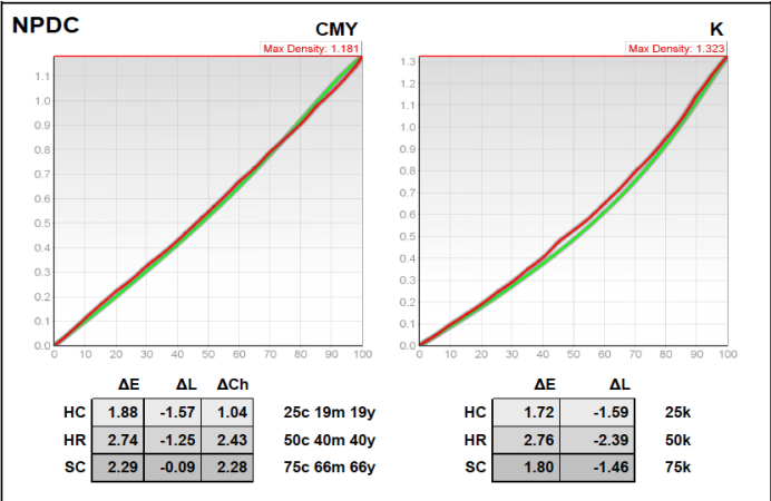
Figure 19: Curve3 results for the Epson 3880 on presentation paper default settings
