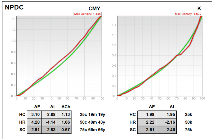
Figure 21: Curve3 results for the Phaser 7880 on plain paper
