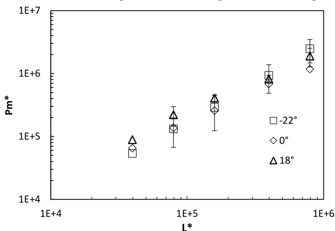
Fig. 11 - Tack vs. line load for different takeoff angles. Experiments use an acrylic web and linseed oil. Optimum web takeoff angle for high tensioned webs is near 0°.
