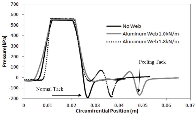
Fig. 4 - Pressure vs. circumferential sensor position for 5 degree web takeoff angle, an aluminum web tensioned at 1.0kN/m or 1.8kN/m with 60.80Pas silicone oil coated at a speed of 0.5m/s.
