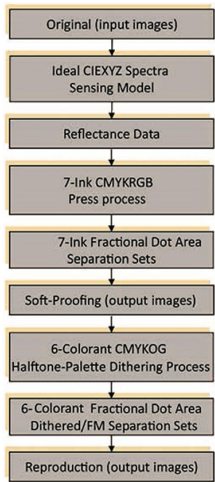
Figure 6: Processes of both FM and halftone-palette half-toning/dithering.
