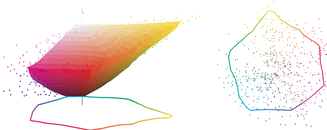
Figure 4: Color Gamut of 12-pt/175lpi print combination
