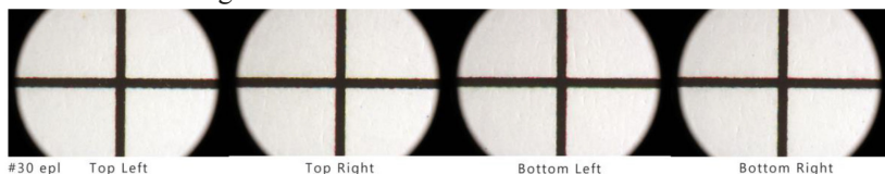
Figure 9. Register marks from four locations from liquid-toner electrophotographic press #30.
