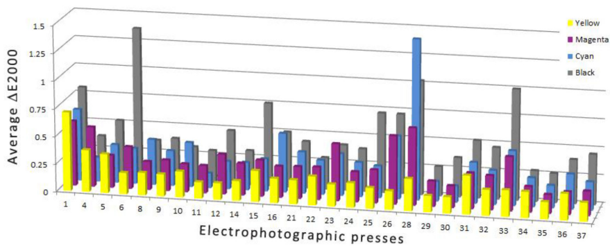
Color Differences for Electrophotographic Presses
