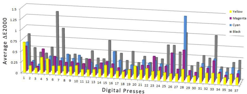
Figure 6. Color differences for process colors across all test form pages and color bar positions.
