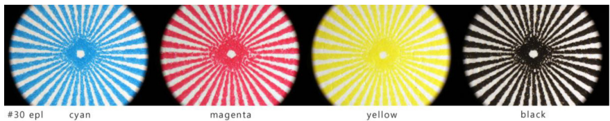
Figure 13. Star Targets with the highest evaluation—liquid-toner electrophotographic (#30).
