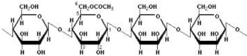
Figure 1: Glucomannan composed of \beta -D-glucopyranose and \beta -D-mannopyranose units linked by 1→4 bonds (second glucopyranose unit is esterified)
