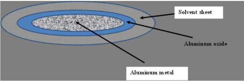
Figure 9: Aluminum flake
