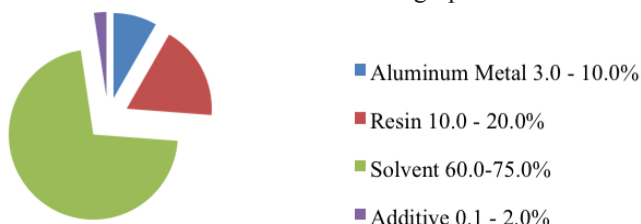
Figure 2: Composition of solvent based dielectric ink
