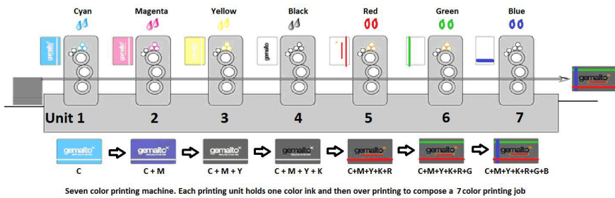
Figure 17: Seven color printing machine
