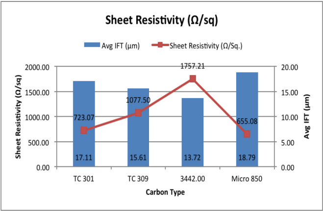
Figure 1: Sheet Resistivity ( \Omega/\text{Sq} ) of four graphite materials, (IFT: Ink Film Thickness)
