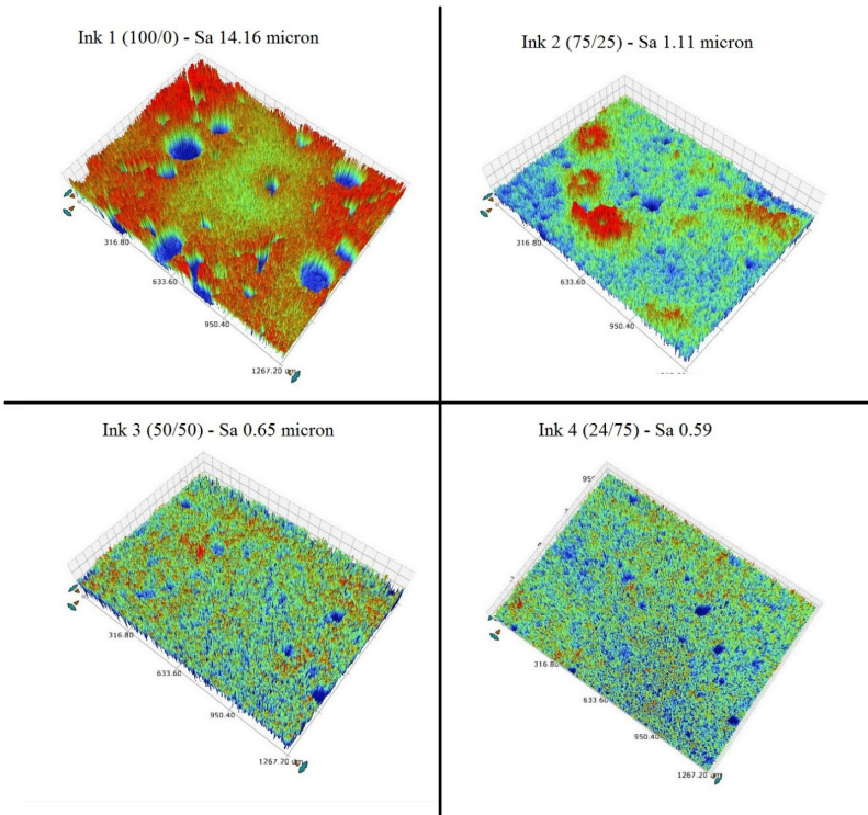
Figure 4: Surface roughness of soy polymer inks
