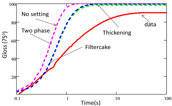
Figure 12. Experimental gloss value and model results of 20% oil diluted ink on a fast setting paper. Model results are predicted for permeability of filtercake K_f = 1.0 \times 10^{-19} \text{m}^2 .
