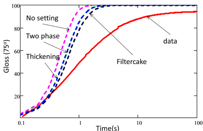
Figure 3. Experimental gloss value and model results of 20% oil diluted ink on a slow setting paper. Model results are predicted for filtercake K_f = 1.0 \times 10^{-16} \text{m}^2 .
