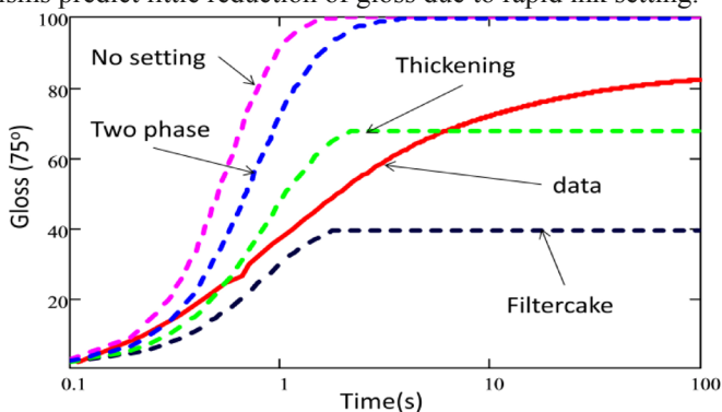
Figure 5. Experimental gloss value and model results of original ink on a slow setting paper. Model results are predicted for filtercake K_f = 1.0 \times 10^{-16} \text{ m}^2 .
