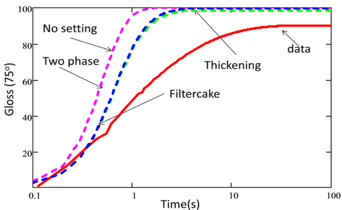
Figure 13. Experimental gloss value and model results of 10% oil diluted ink on a fast setting paper. Model results are predicted at permeability of filtercake K_f = 1.0 \times 10^{-19} \text{m}^2 .
