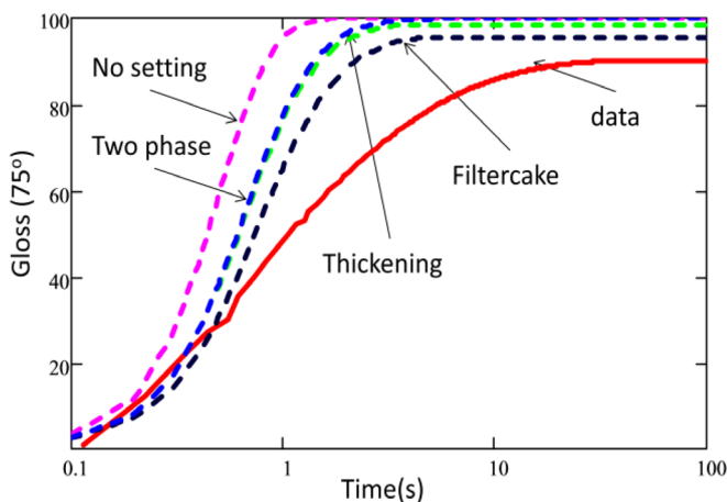
Figure 6. Experimental gloss value and model results of 20% oil diluted ink on a fast setting paper. Model results are predicted for filtercake K_f = 1.0 \times 10^{-16} \text{ m}^2 .
