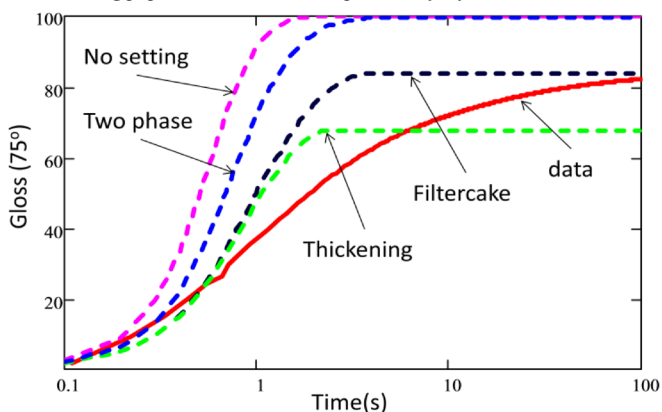
Figure 11. Experimental gloss value and model results of the original ink on a slow setting paper. Model results are predicted for filtercake K_f = 1.0 \times 10^{-10} \text{ m}^2 .
