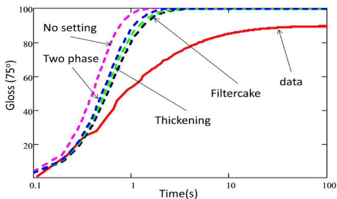
Figure 10. Experimental gloss value and model results of 10% oil diluted ink on a slow setting paper. Model results are predicted for filtercake K_f = 1.0 \times 10^{-10} \text{ m}^2 .
