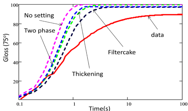
Figure 4. Experimental gloss value and model results of 10% oil diluted ink on a slow setting paper. Model results are predicted for filtercake K_f = 1.0 \times 10^{-16} \text{m}^2 .
