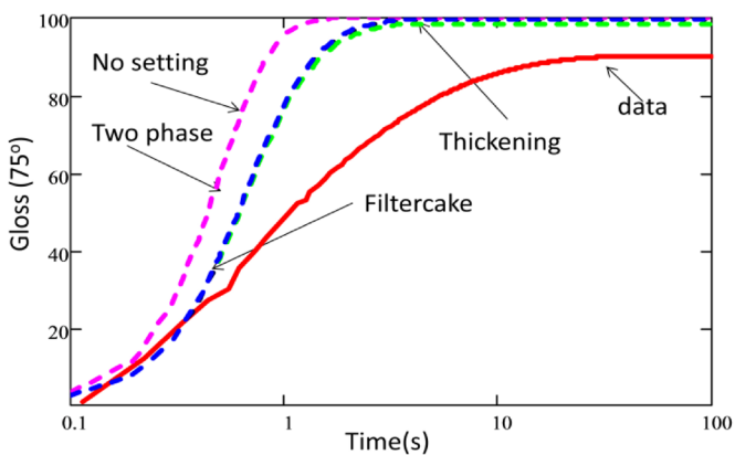
Figure 14. Experimental gloss value and model results of pure ink on a fast setting paper. Model results are predicted at permeability of filtercake K_f = 1.0 \times 10^{-19} \text{m}^2 .
