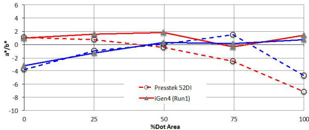
Figure 5. Gray reproduction comparison between Presstek 52DI and iGen4
