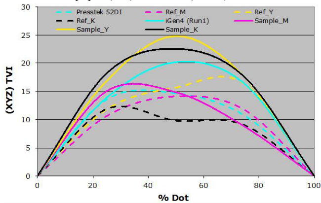
Figure 6. TVI comparison between Presstek 52DI (reference) and iGen4
