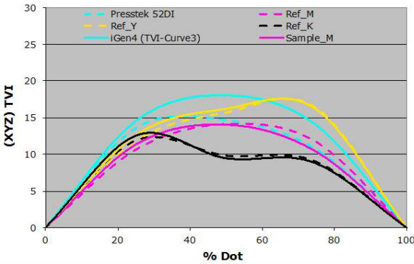
Figure 13. Using Curve3 to implement the TVI adjustment method
