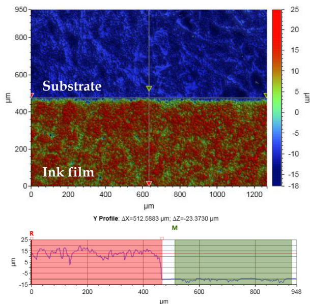
Figure 8. Profilometry scan of ink film and substrate
