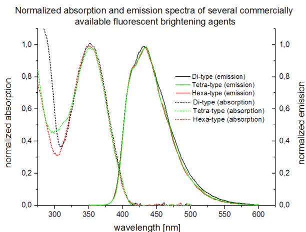
Figure 12: Normalized absorption and emission spectra of several FBAs solved in H 2 O. Common emission maxima at 435nm and common absorption maxima at 350nm are obtained. Differences in local minima are found in the range of 275-325nm
