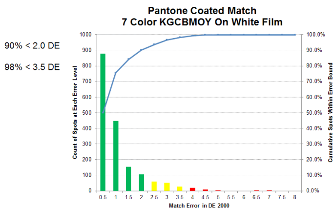
Figure 22. Pantone color matching results for the KGCBOY configuration.
