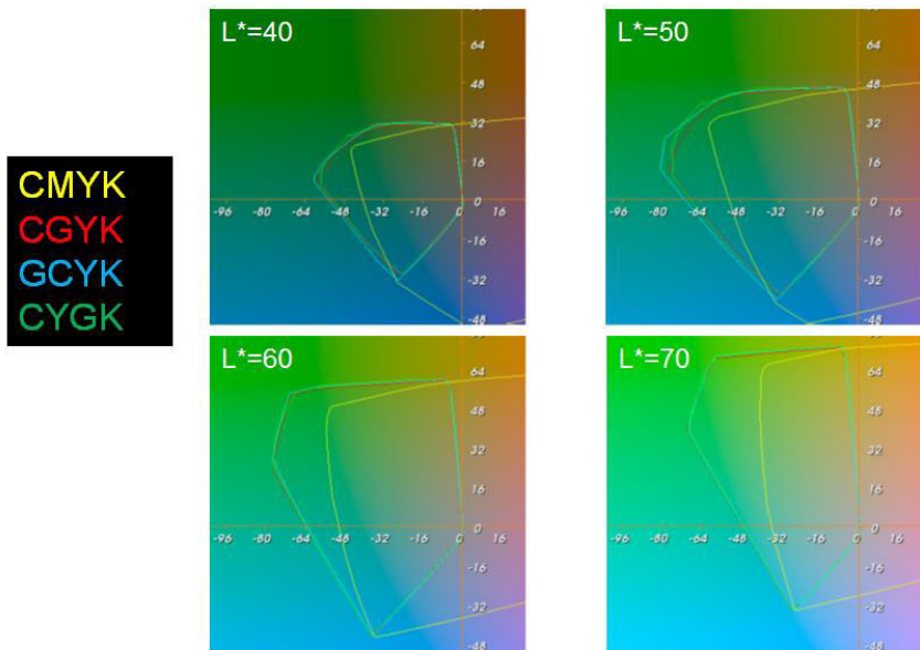
Figure 12. Color gamut slices for CGYK, GCYK, and CYGK compared to the reference CMYK ink set.
