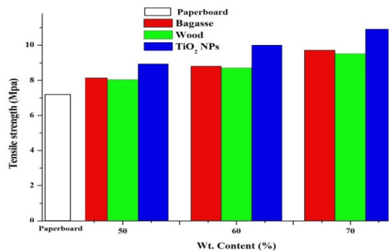
Fig. 2 Tensile strength of coated and uncoated paperboard samples.
