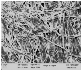
Fig 1. (a) SEM image of uncoated paperboard sample.
