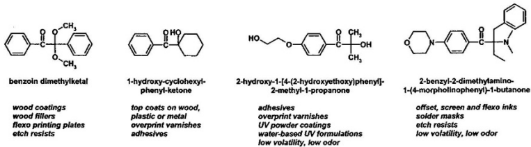
Figure 4: Structure of typical photo initiators and their main application areas (Dietliker et al. 2004, S. 78)
