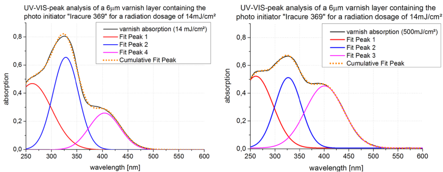
Figure 13: UV-VIS analysis of the absorption spectra of a 6µm varnish layer containing 1% of the photo initiator „Irgacure 369” solved in 80% “TPGDA” and 19% “LEO10801” for radiation doses of 14mJ/cm² (left) and 500mJ/cm² (right)
