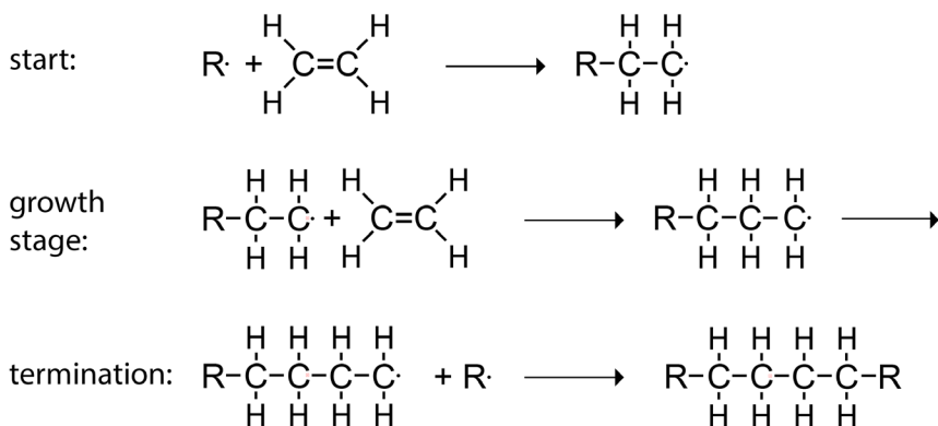
Figure 1: Stages of the radical polymerization process
