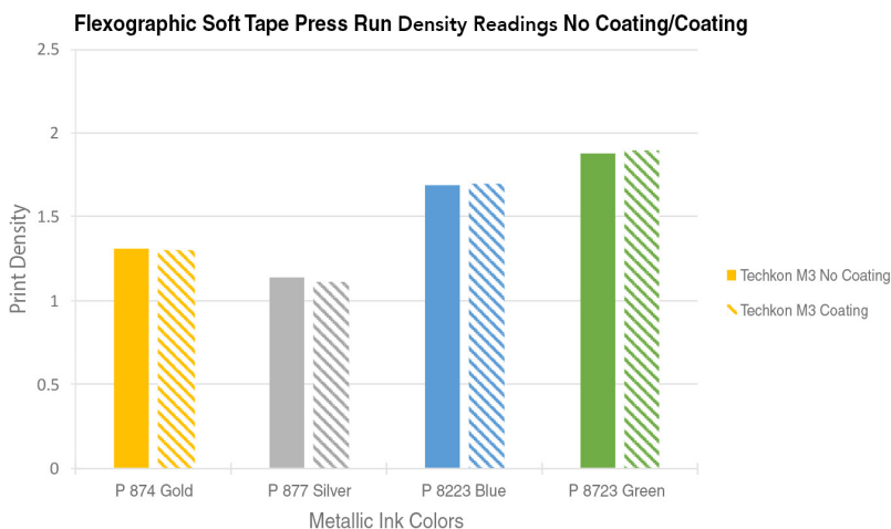
Figure 20: A comparison of the gloss-coated and non-coated print density values from flexographic soft tape press run with the SpectroDens in M3 mode
