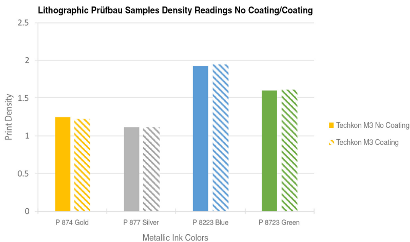
Figure 25: A comparison of the gloss-coated and non-coated print density values from the lithographic Prüfbau samples with the SpectroDens in M3 mode
