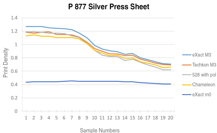
Figure 8: Printed ink density measurements of the four devices of P 877 silver press run sheets
