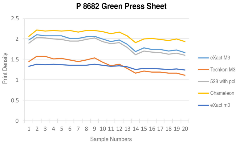
Figure 11: Printed ink density measurements of the four devices of P 8682 green press run sheets
