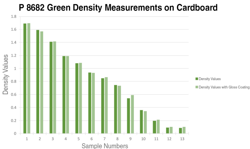
Figure 13: A comparison of gloss-coated and non-gloss coated density measurements of P 8682 green, Prüfbau samples with X-Rite eXact M3 mode
