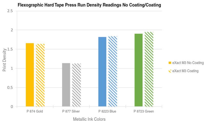
Figure 23: A comparison of gloss-coated and non-coated print density values from flexographic hard tape press run with the eXact in M3 mode
