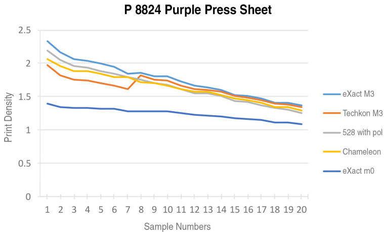
Figure 10: Printed ink density measurements of the four devices of P 8824 purple press run sheets
