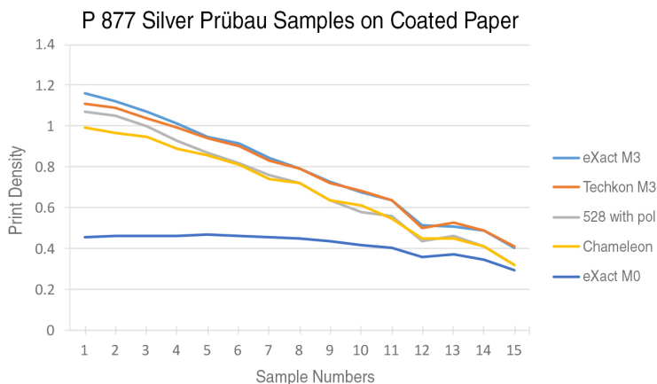
Figure 1: The density measurements of P 877 Silver Prüfbau samples with the eXact (M3, M0), SpectroDens (M3), 528 and Chameleon
