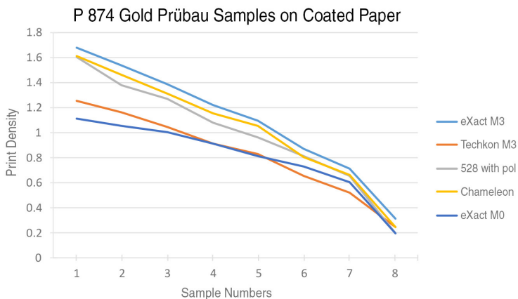
Figure 2: The density measurements of P 874 Gold Prüfbau samples with the eXact (M3, M0), SpectroDens (M3), 528 and Chameleon
