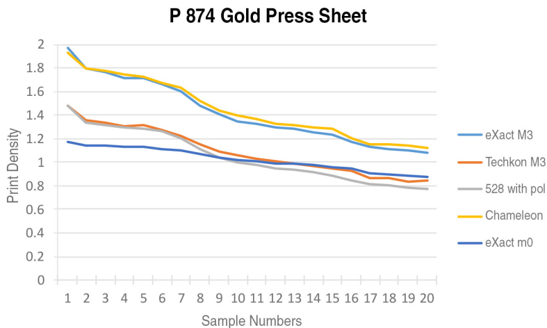
Figure 9: Printed ink density measurements of the four devices of P 874 gold press run sheets
