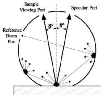
Figure 3. Schematic of an Integrating Sphere Instrument
