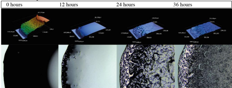
Figure 4: Time dependence images from the laser scanning microscope of a drying 1 \mu\text{l} ethylene glycol drop on glass after (Image size: 1,4x1mm 2 )
