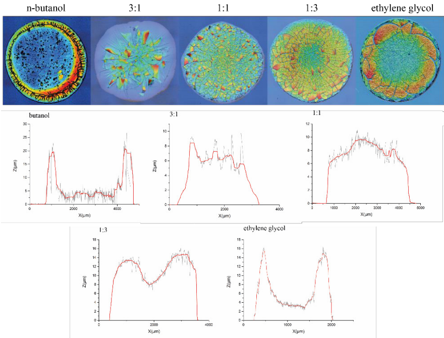
Figure 2: Overview of the variation of 1ul butanol- ethylene glycol mixtures on glass which show different profiles of height. Coffee-Stain Effect: 1-butanol, 1:3 and ethylene glycol; aggregation at the center: 3:1; uniform profile:1:1
