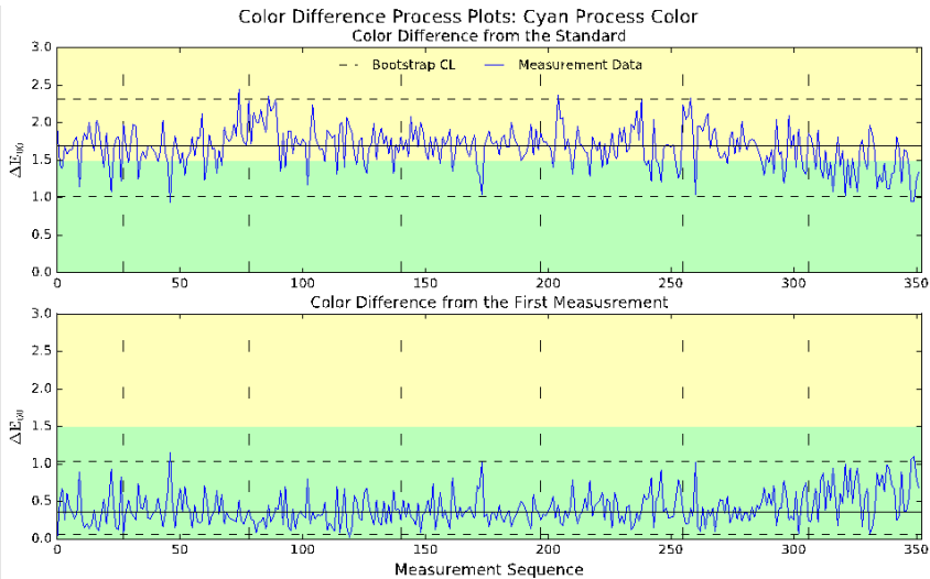
Figure 1. Color difference data process data for a cyan process color. Top) Color difference from the standard, \Delta E_{00(S)} , and Bottom) Color difference from the first measurement, \Delta E_{00(D)} . The upper and lower control limits were calculated using a bootstrap method proposed by Phaladiganon, et al. (2009).
