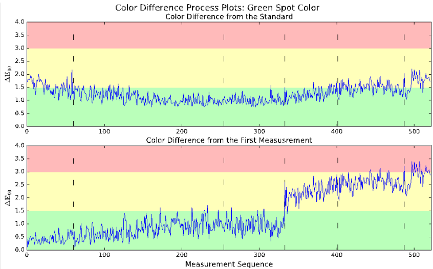
Figure 2. Color difference data process data for a green spot color. Top) Color difference from the standard, \Delta E_{00(S)} , and Bottom) Color difference from the first measurement, \Delta E_{00(D)} .
