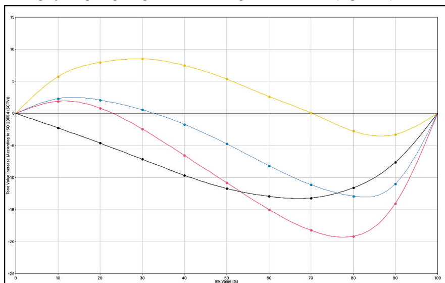
Figure 10. CTV curves after G7® gray balance correction: inkjet printer
