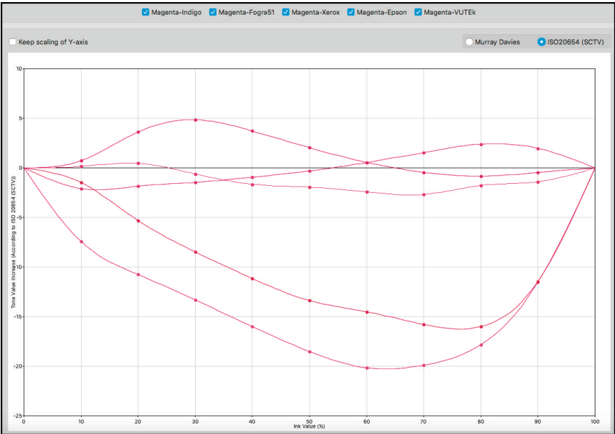
Figure 9. CTVI curves of 5 printing systems
