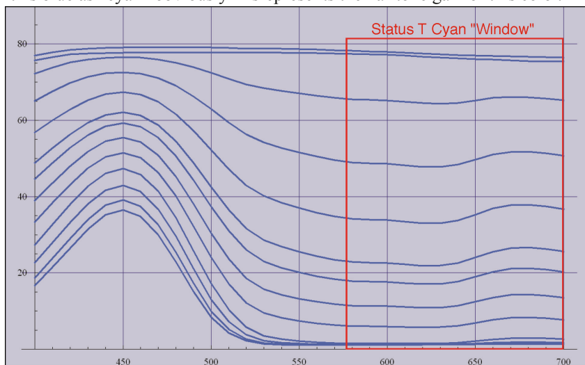
Figure 1. Spectra of tone curves of reflex blue showing inaccurate Status T definition as process cyan (Courtesy John Seymour)
