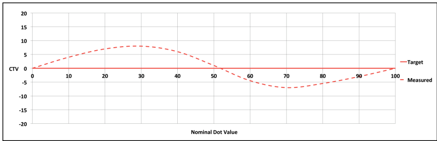
Figure 3. Newer style graph showing horizontal line as CTVI target
