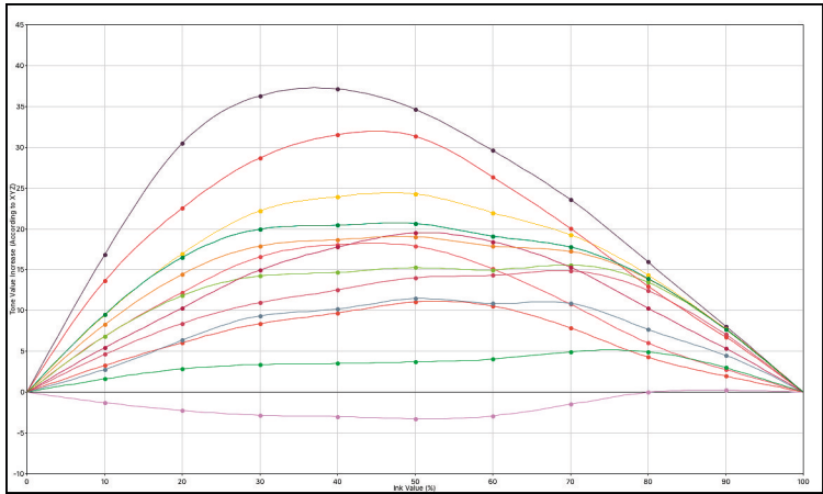
Figure 2. TVI of 13 spot colors
