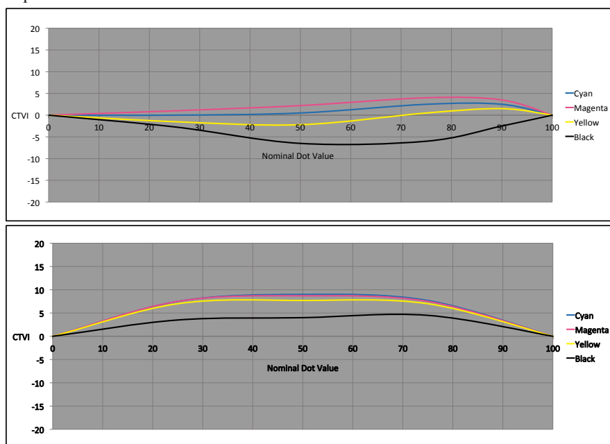
Figure 12. CTV curves of GRACoL2013 CRPC6 (top) and Fogra 52 (bottom)
