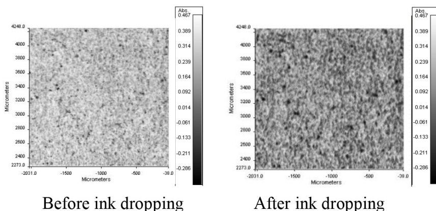
Figure 3. Two-dimension images of the carbonyl group (1730 cm -1 ) before and after UV curable ink dropping
