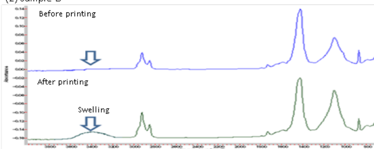
Figure 7. ATR spectra of blankets before and after printing (1) Sample A, (2) Sample B
