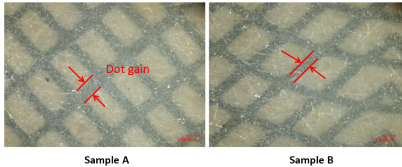
Figure 10. Optical microscope images of lines printed using Sample A and Sample B
