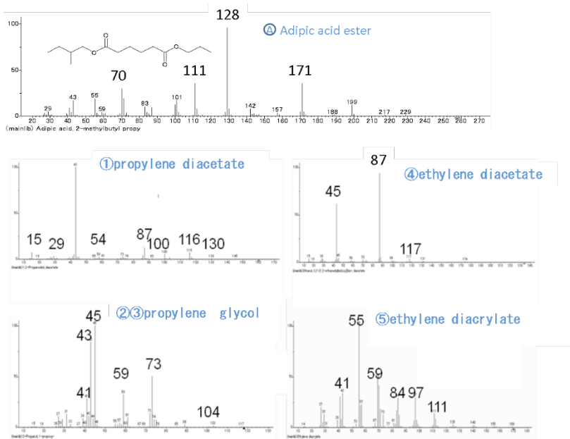
Figure 5. MS spectra identified each peak in Figure 4
