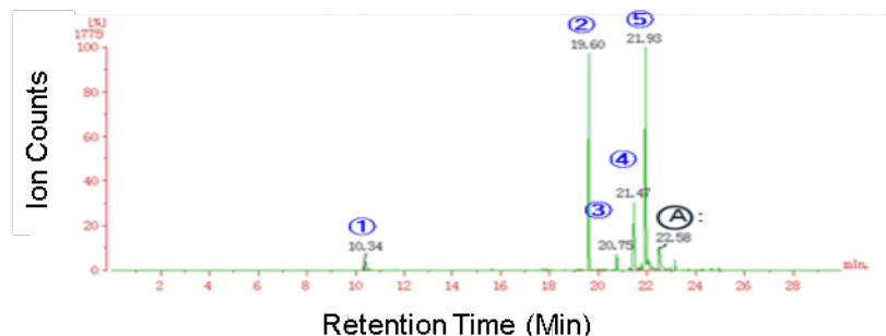
Figure 4. TIC of extract with petroleum ether of sample B
