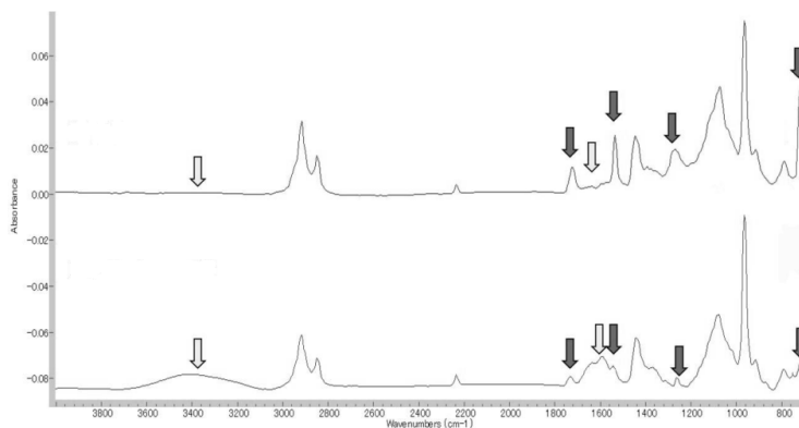
Figure 1. ATR spectra of rubbers before and after dropping the UV curable ink on the surface of sample A
