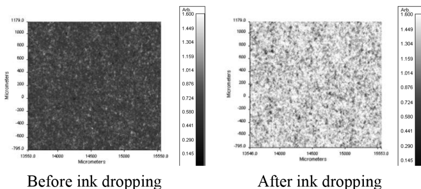
Figure 2. Two-dimension images of the hydroxyl group (3400 cm -1 ) before and after UV curable ink dropping
