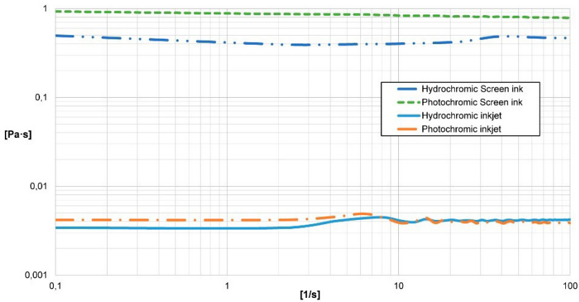
Figure 7: Flow behavior screen-printing and inkjet inks
