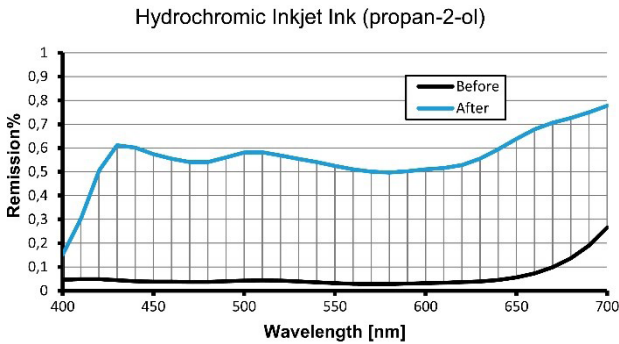
Figure 5: Spectral analysis pattern of the hydrochromic inkjet ink
