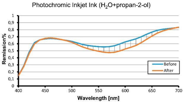
Figure 6: Spectral analysis pattern of the photochromic inkjet ink
