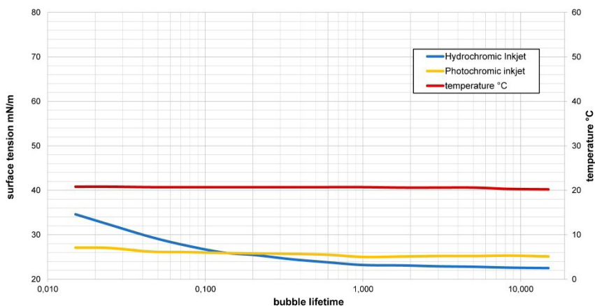
Figure 8: surface tension of developed inkjet inks
