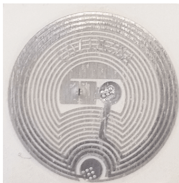
Figure 1.1 NFC “Tag” on adhesive side of a Product Label
