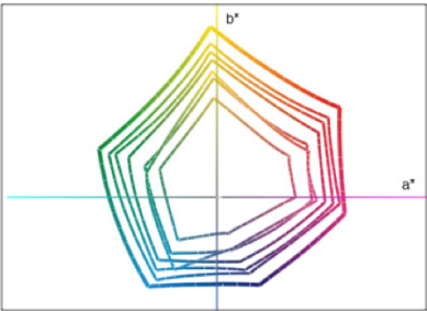
Figure 1. Seven CRPCs and corresponding gamut sizes.
