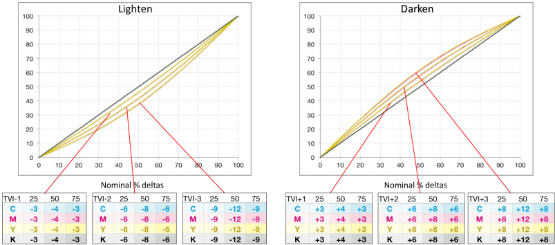
Figure 7. Tonality Adjustments as Tone Curves.
