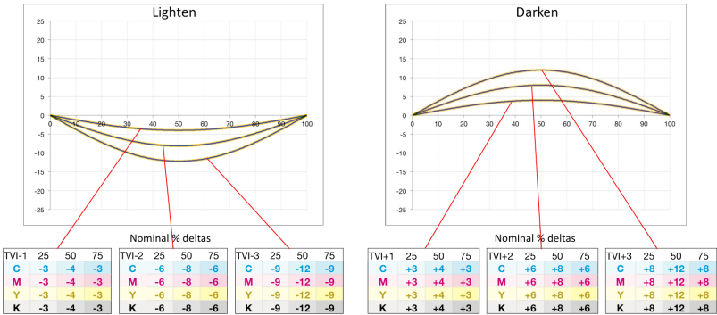
Figure 6. Tonality Adjustments as TVI.
