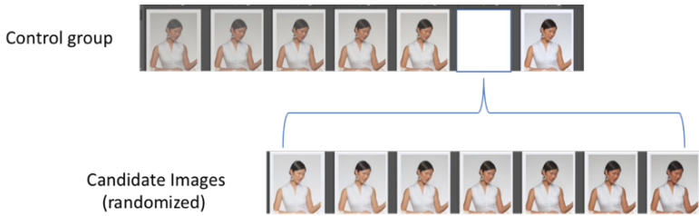
Figure 17. A procedure for the psychometric test: “There is a ‘hole’ in the (Control) group of images. Rank the candidate images according to the resulting consistency of color appearance of the group when a candidate image fills the gap, from the highest to the lowest.”
