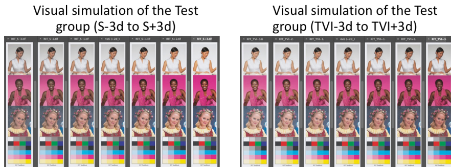
Figure 19. Visual simulation for the datasets varying in tonality.
