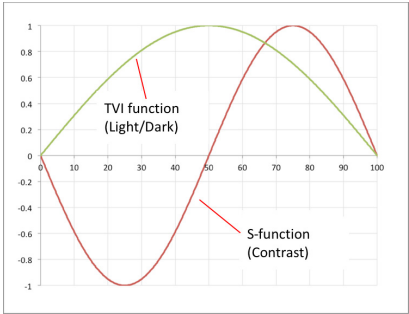
Figure 5. TVI and S-curve functions.
