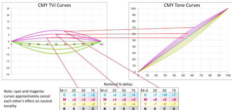
Figure 14. Magenta-Biased Gray Balance Adjustments
