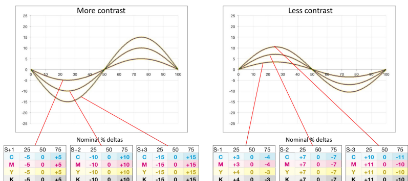
Figure 8. Contrast modifications(S-Curve) as TVI.
