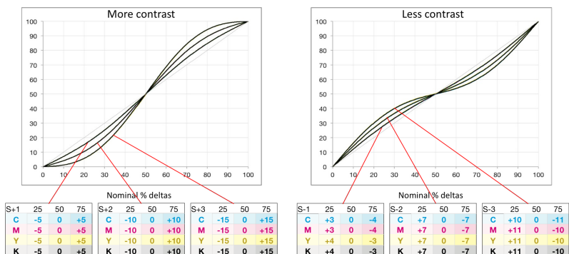
Figure 9. Contrast modifications(S-Curve) as Tone Curves.
