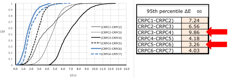
Figure 4. Cumulative Relative Frequency of \Delta E_{00} (CRF) and the 95 th percentile \Delta E_{00} for adjacent CRPCs.
