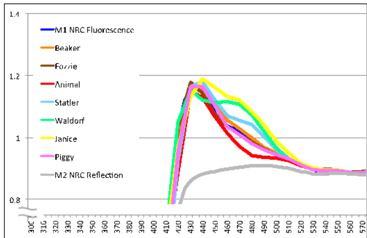
Figure 04: expanded view 'Region of Interest' McCoy 80lb M1 - Normalized to 560nm
