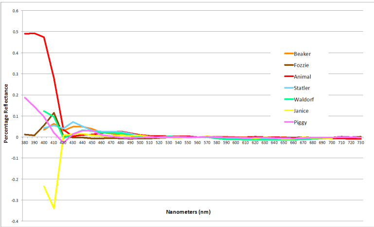
Figure 09: McCoy 80lb M2 Normalized – Difference to NRC
