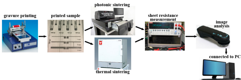
Figure 4. Experiment setup
