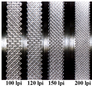
Figure 3. Different line screens on gravure plate
