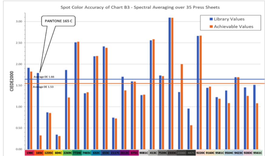
Figure 7: Spot color accuracy of chart location B3 – spectral averaging over 35 sample sheets.
