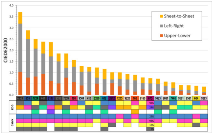
Figure 24: Color separation using ECG versus CMYK.
