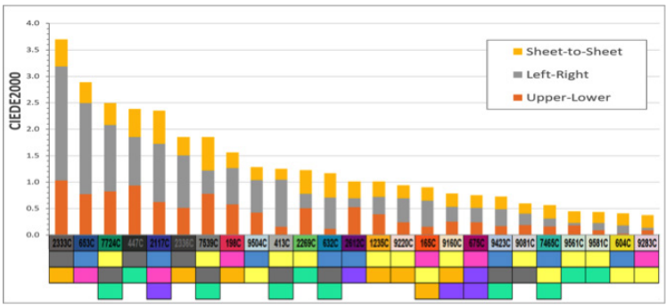
Figure 23: Color separation used when converting the 25 spot colors into ECG.
