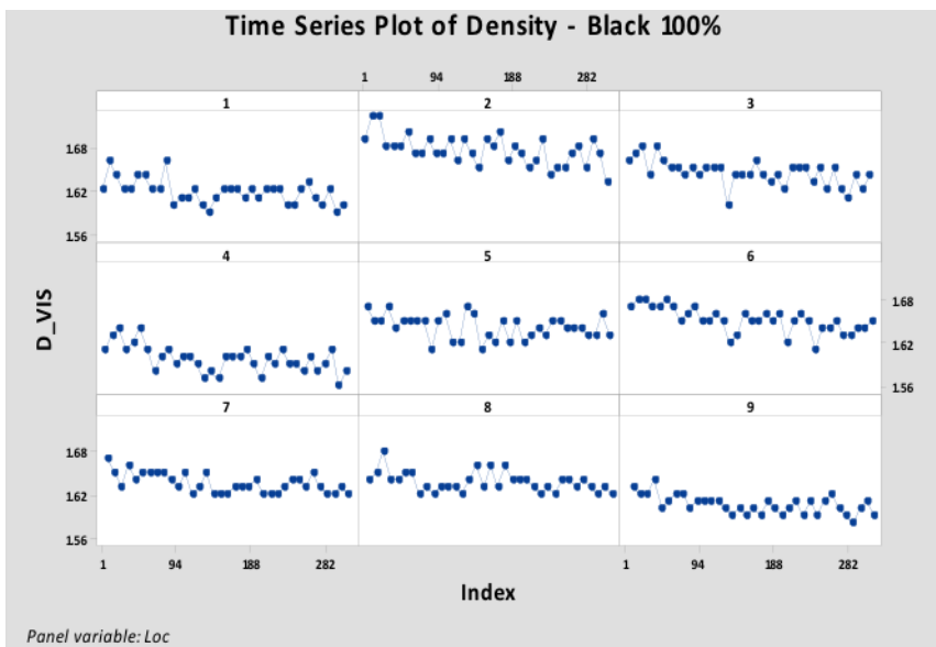
Figure 20: Density variation of the black printing unit based on locations.
