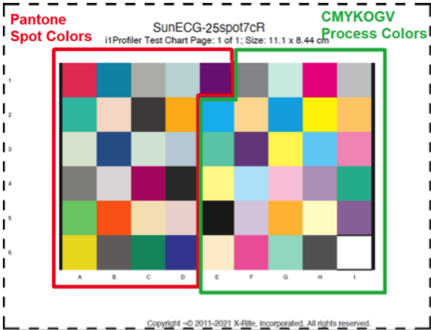
Figure 3: The colors in figure 2 are randomized and put into a test chart format suitable for i1iO. The chart was then placed into the press form layout.
