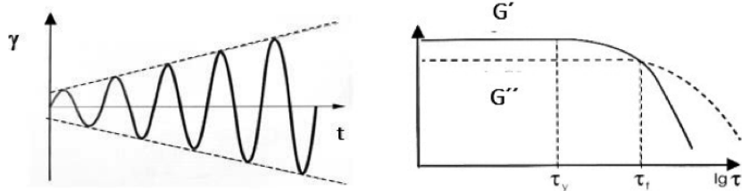
Figure 8. Adapted from [16]: Amplitude sweep. Figure 9. Adapted from [16]: Limit of LVE region.
