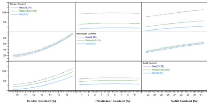
Figure 32. Interaction graphs. Shear viscosity at shear rate 50.
