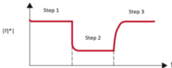
Figure 13. Creep and Recovery test.
