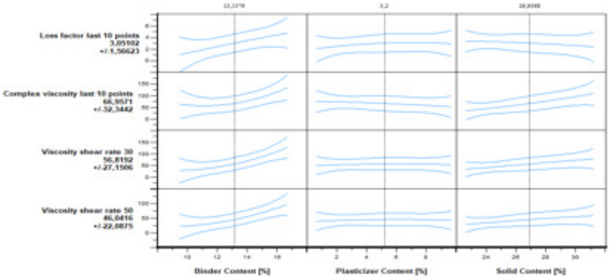
Figure 35. Predicted response graph, Profile I.
