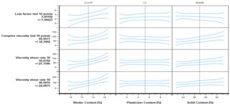
Figure 36. Predicted response graph, Profile II.
