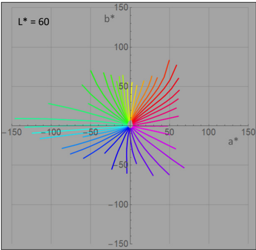
Figure 6 – Spidergram showing hue differences between CIELAB and NCS at an L^* near 60
