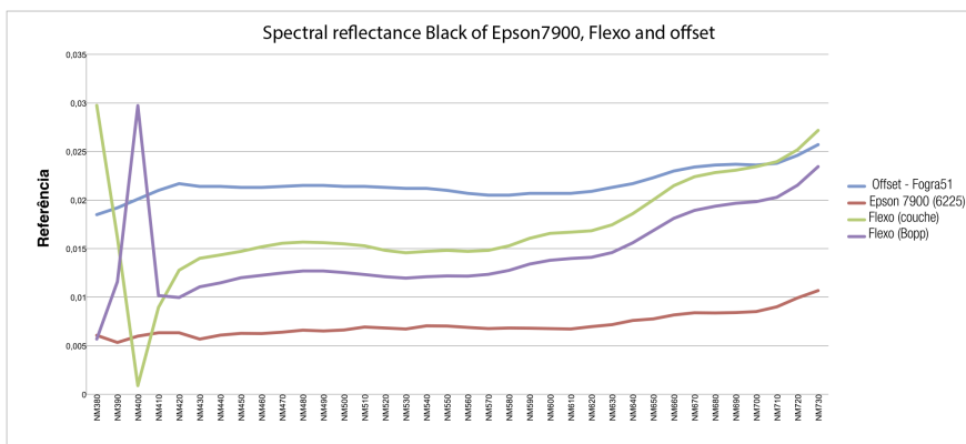
Figure 3d. Comparison of the spectral curve energy distribution of black in analogic processes versus inks used by Epson 7900.
