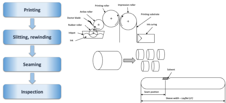
Figure 1. Heat-shrinkable labels production process
