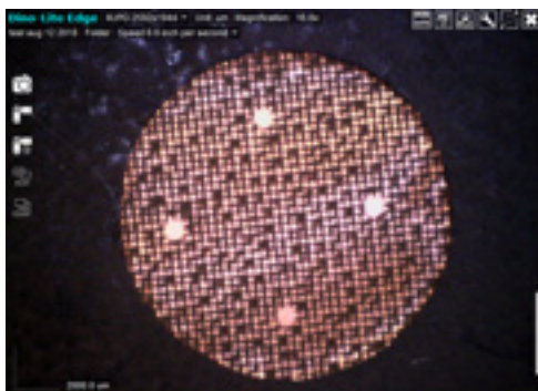
Figure 8 : Detail of print on 75 LPI plate with 500 \mu\text{m} nonimage area SG/C45/5130- 90/3/7 at 33% SC
