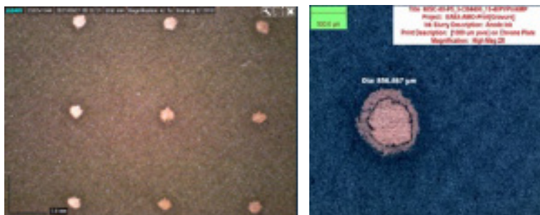
Figure 9: Detail of NMP ink with PVP resin showing print with 1000 \mu\text{m} non image areas
