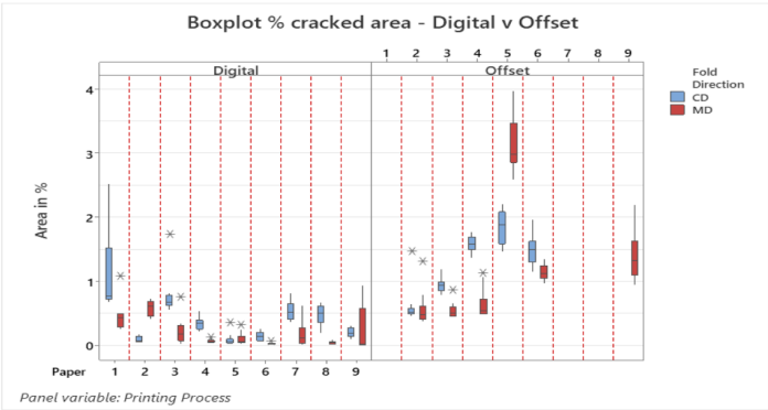
Fig. 8: Degree of cracking in MD and CD
