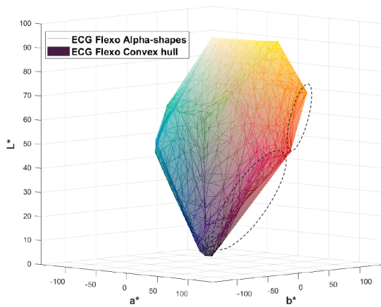
Figure 1. Visualization of two gamuts computed from the same data set of ‘ECG Flexo’ using the alpha-shapes and the convex hull methods in the CIELAB color space. Below are the results comparing ECG Flexo against other gamuts for each of the use-cases.
