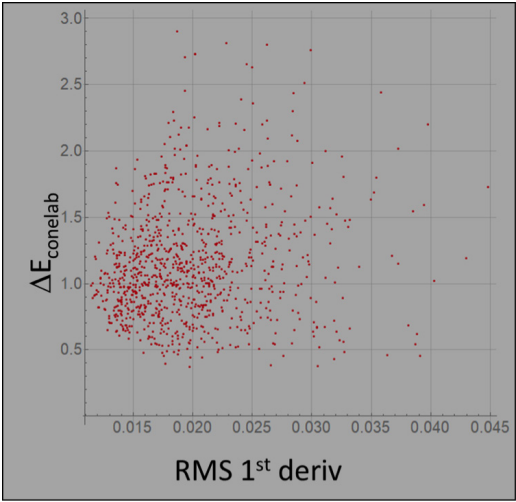
Figure 5 – Color inconstancy of metamers as a function of average first derivative
