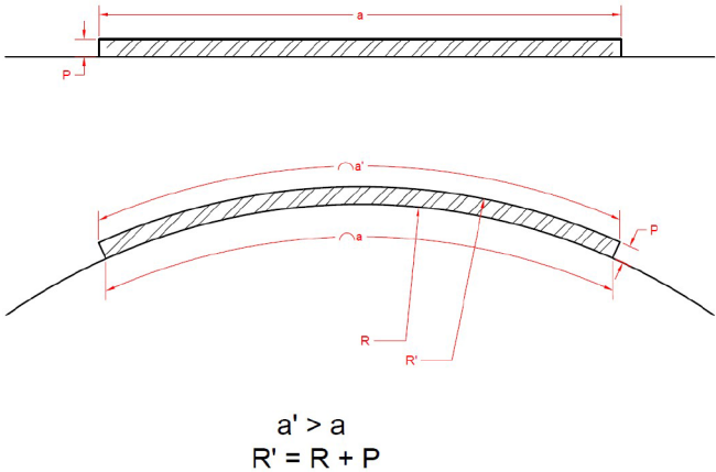
Figure 10: Plate surface elongation when it is curved.
